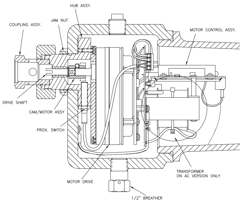
Figure 1.1—CD-20SFA controller components
