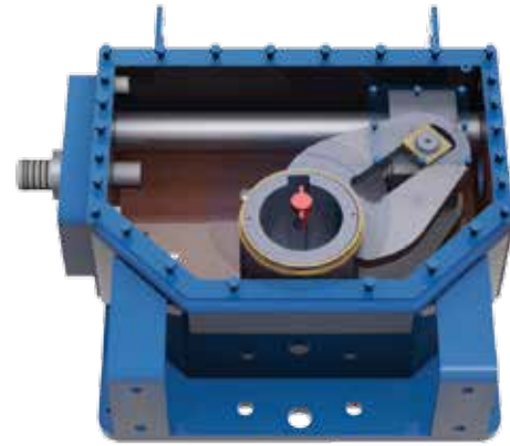
Fabricated Frame
